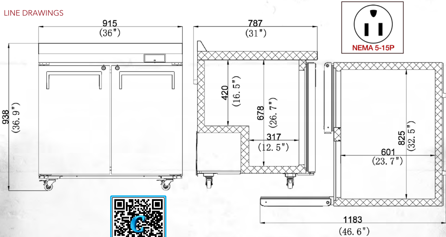
PRODUCT DRAWINGS
